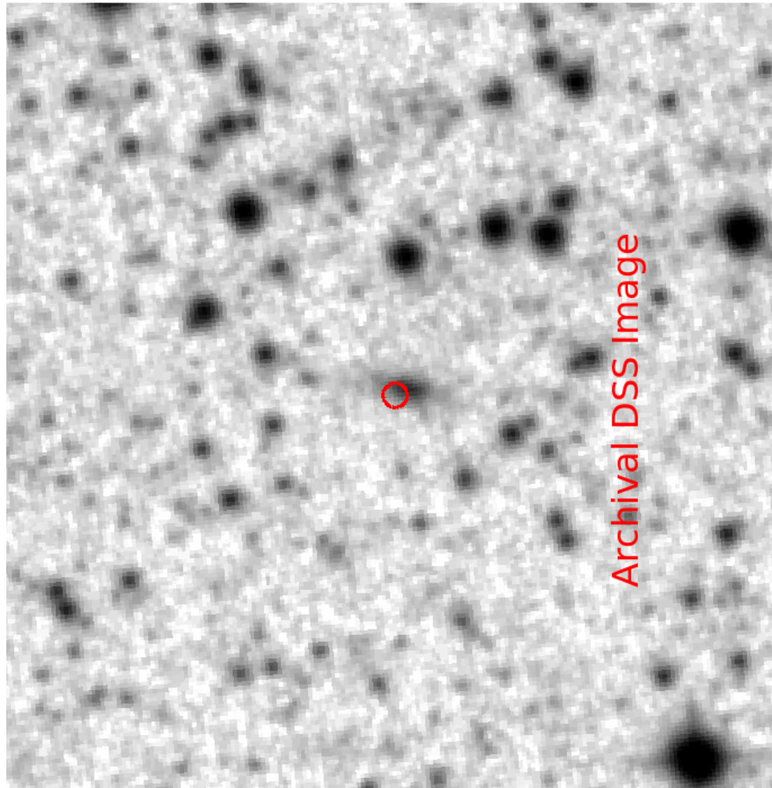
ASASSN-15ps 2015-09-18 Confirmation
